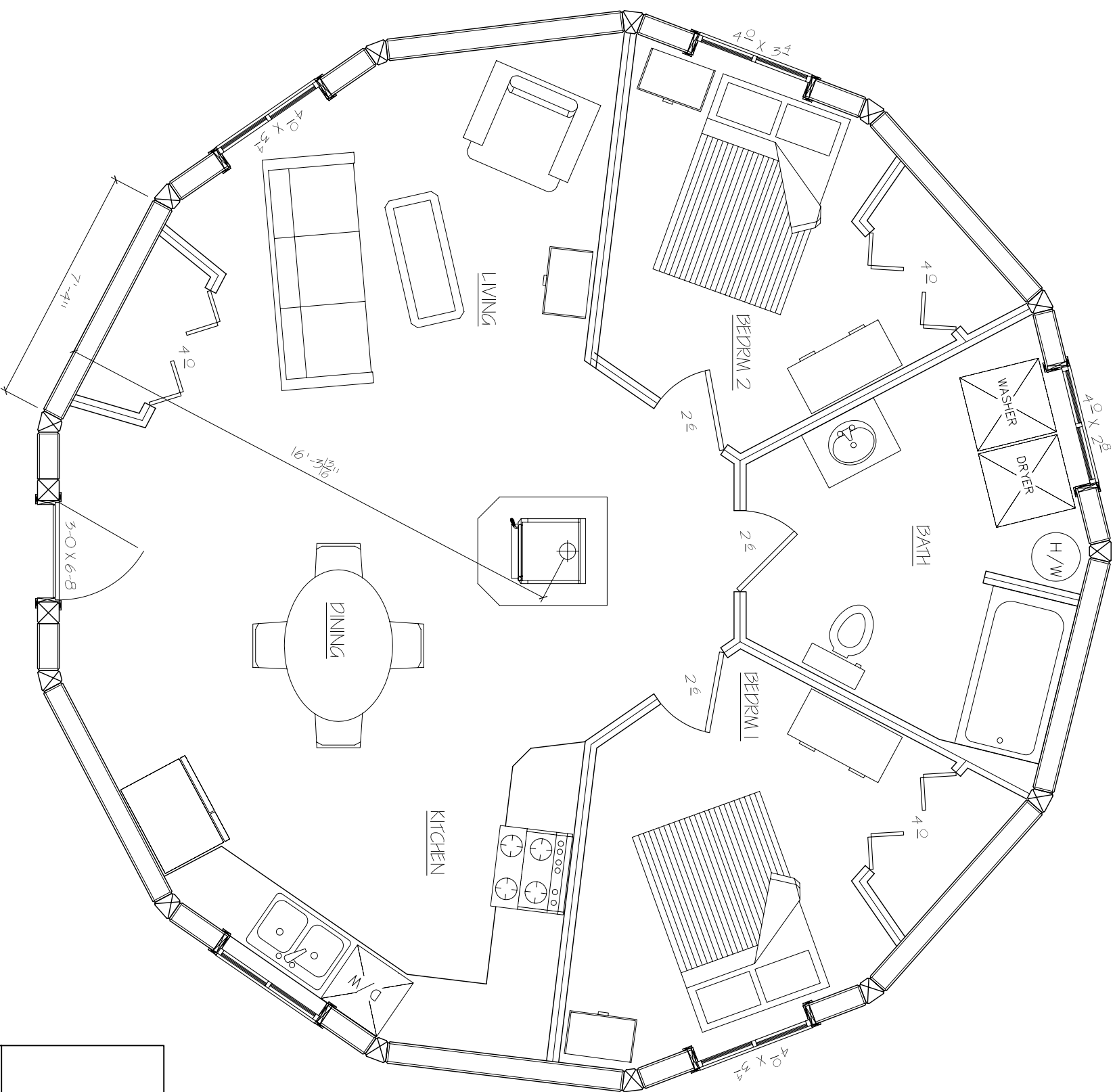
FLOOR PLAN FLOOR AREA 853 SQ-FT
